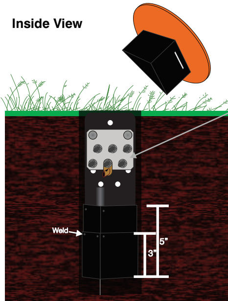
Grounded LocatePlate
